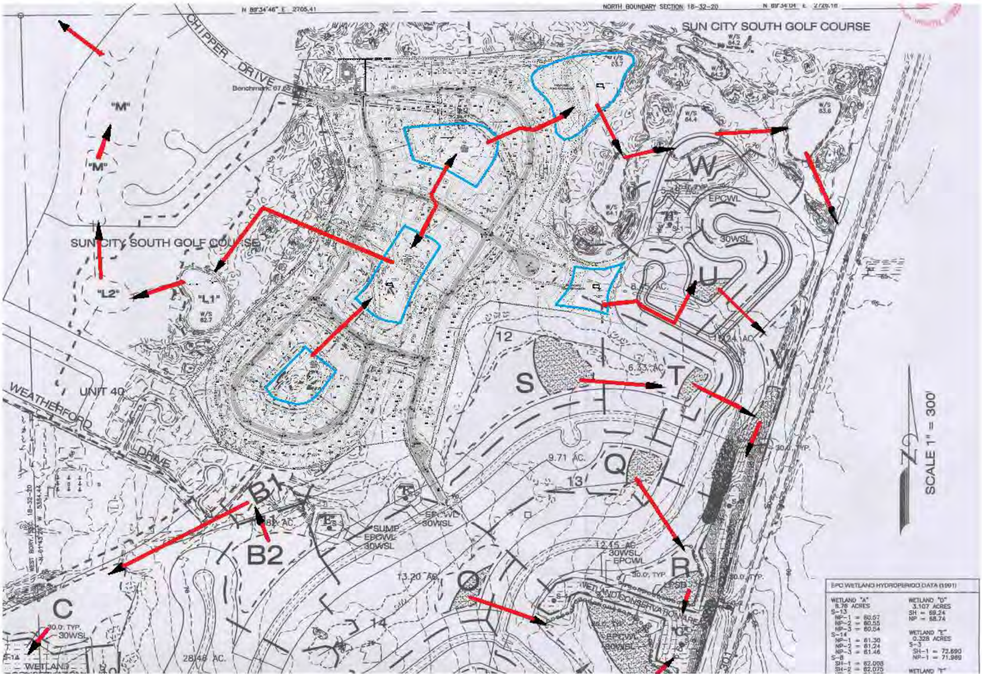
VERONA OVERLAID ONTO ORIGINAL MASTER DRAINAGE PLAN
